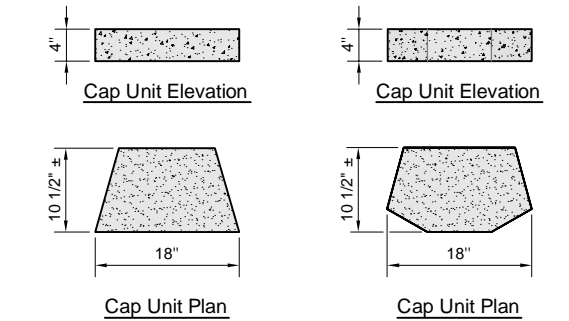
Universal Cap Unit Option *Dimensions & Availability Will Vary by Region 3-Plane Split Cap Unit Option *Dimensions & Availability Will Vary by Region
