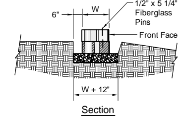
Leveling Pad Detail
