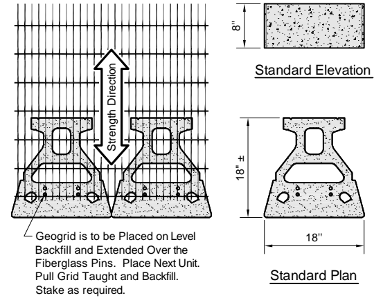
Grid & Pin Connection
