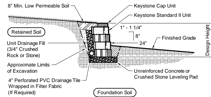
Typical Gravity Wall Section Standard II Unit - 1\"/>
