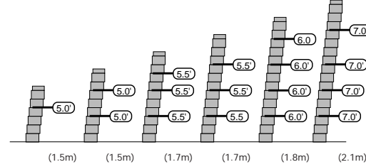
► Geogrid Placement Chart
