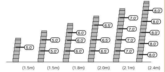
► Geogrid Placement Chart
