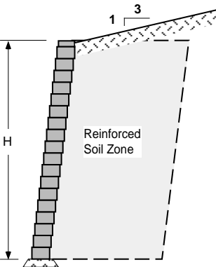
► Geogrid Placement Chart
