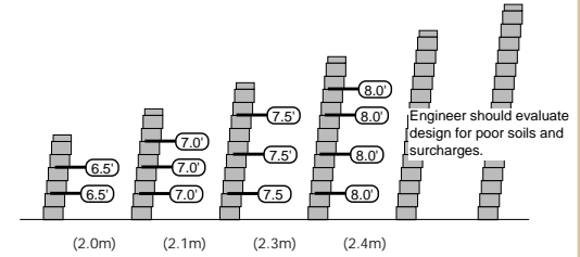
► Geogrid Placement Chart
