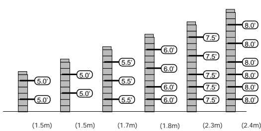
► Geogrid Placement Chart
