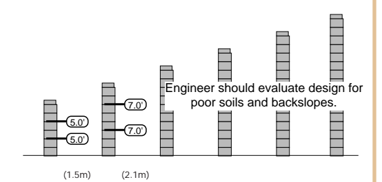
► Geogrid Placement Chart
