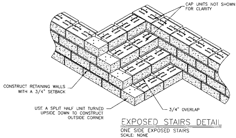
EXPOSED STAIRS DETAIL ONE SIDE EXPOSED STAIRS SCALE: NONE
