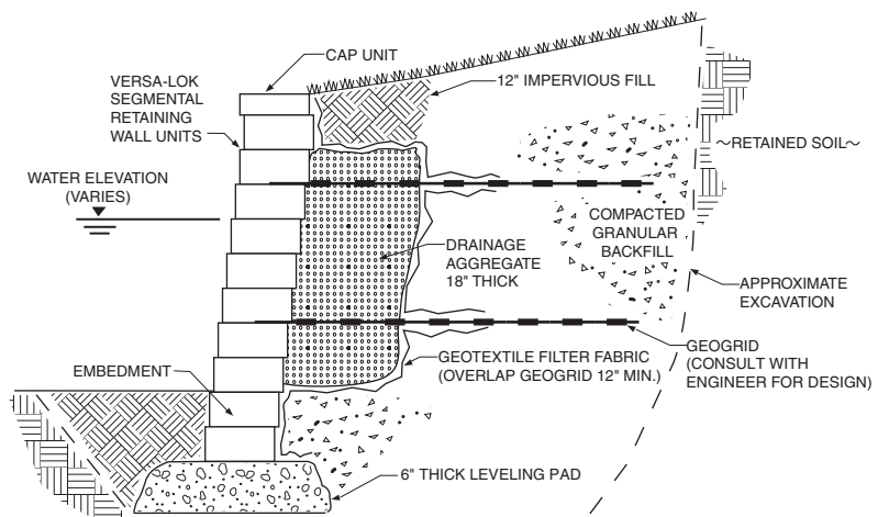
FIGURE 1 Retention Pond — Typical Section (scale: none)
