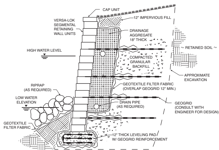
FIGURE 2 Shore Protection — Typical Section (scale: none)
